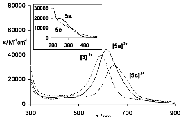
Figure 7. Electronic absorption spectra (CH 2 Cl 2 ) of [3] 2+ (···), [5a] 2+ (—), [5c] 2+ (·-·), inset shows the spectra for 5a (—) and 5c (·-·).
